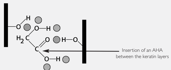
Example of a potential hydrogen bond
