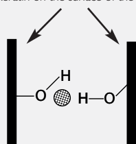
Hydrogen bonds
